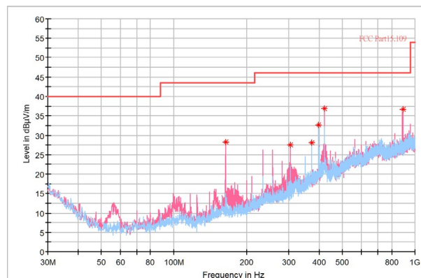
Figure 8. 30M-1GHz
