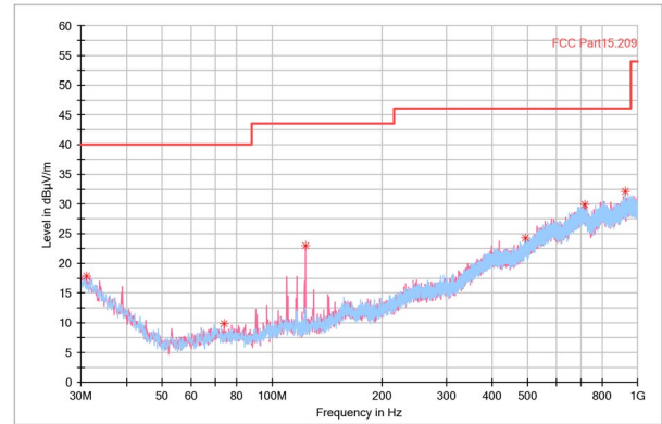
Figure 2. 30M-1GHz
