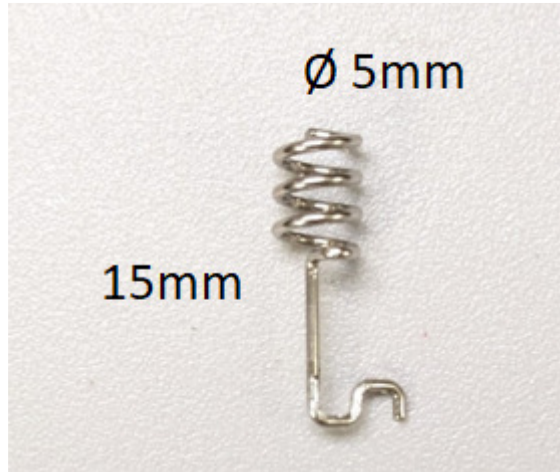
Figure 1 Physical dimension (mm)
