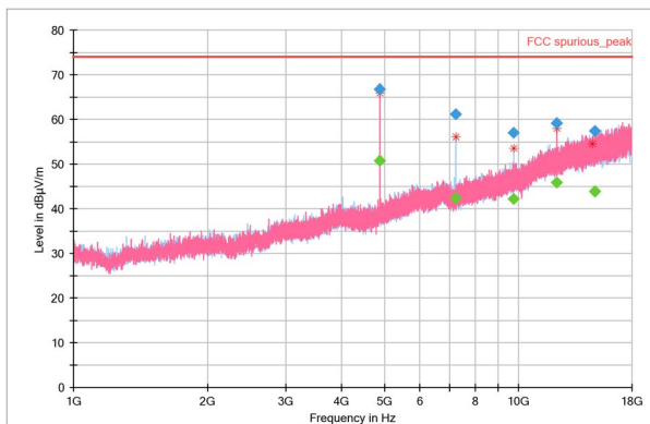
Figure 3. 1-18GHz Peak
