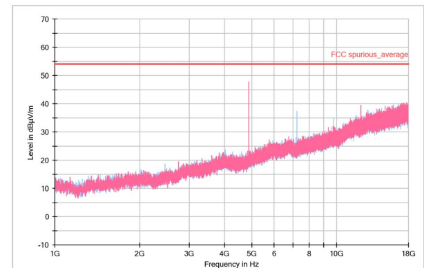
Figure 4. 1-18GHz Average
