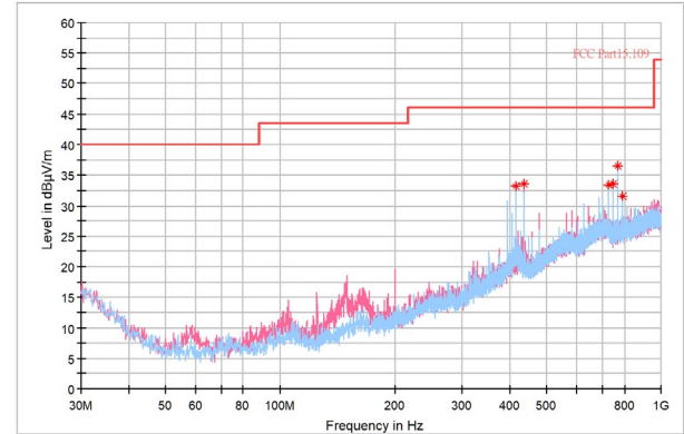
Figure 2. 30M-1GHz
