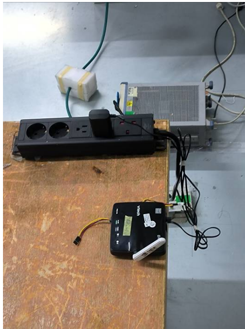
Conducted Emissions - Side View
