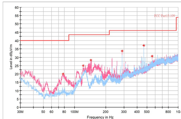
Figure 15. 30M-1GHz
