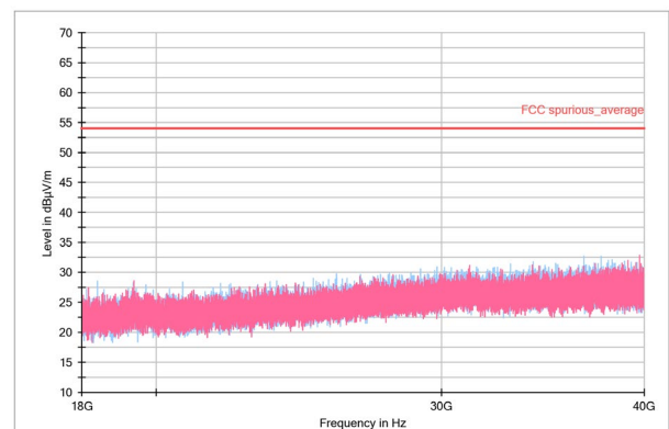
Figure 6. 18-40GHz Average
