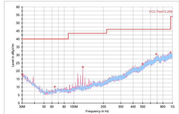
Figure 8. 30M-1GHz
