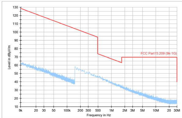
Figure 7. 9k-30MHz
