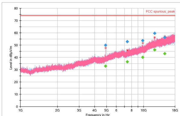
Figure 10. 1-18GHz Peak
