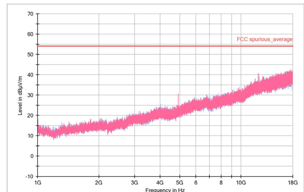
Figure 11. 1-18GHz Average
