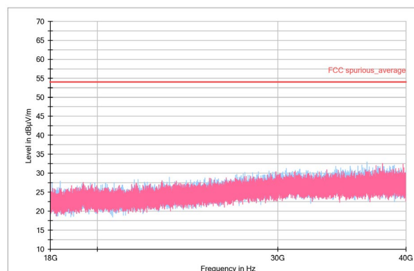
Figure 13. 18-40GHz Average
