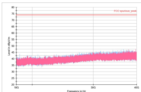
Figure 12. 18-40GHz Peak
