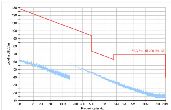
Figure 14. 9k-30MHz
