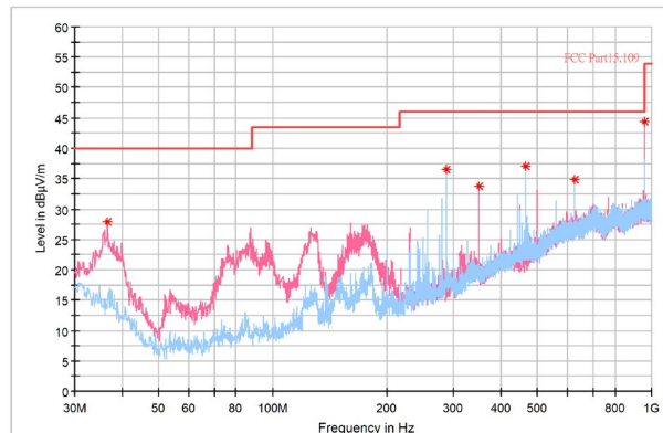
Figure 8. 30M-1GHz
