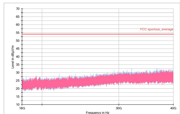
Figure 6. 18-40GHz Average
