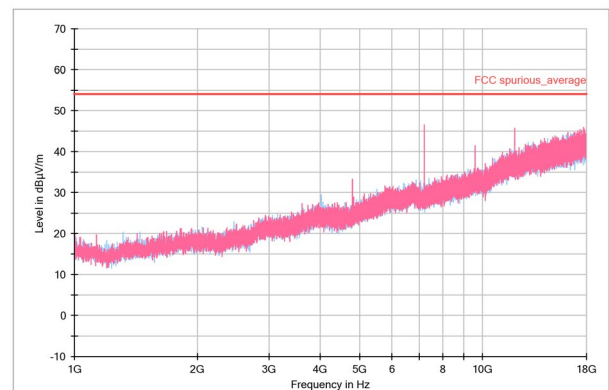
Figure 4. 1-18GHz Average
