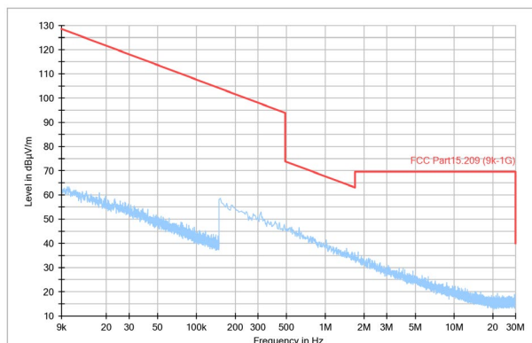
Figure 7. 9k-30MHz
