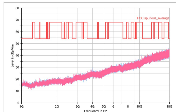
Figure 5. 1-18GHz Average
