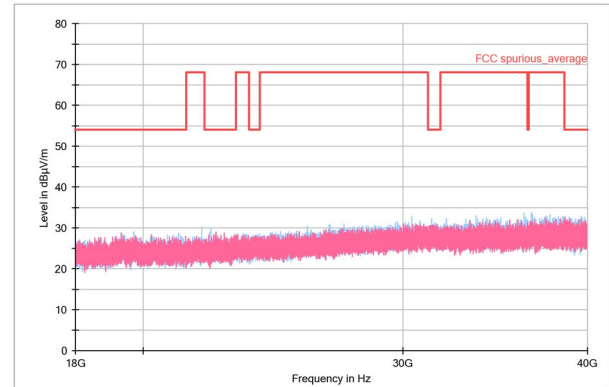
Figure 7. 18-40GHz Average
