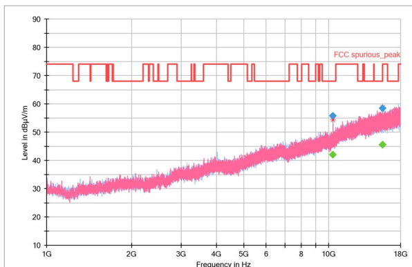
Figure 4. 1-18GHz Peak
