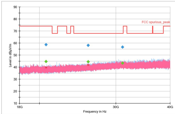
Figure 6. 18-40GHz Peak
