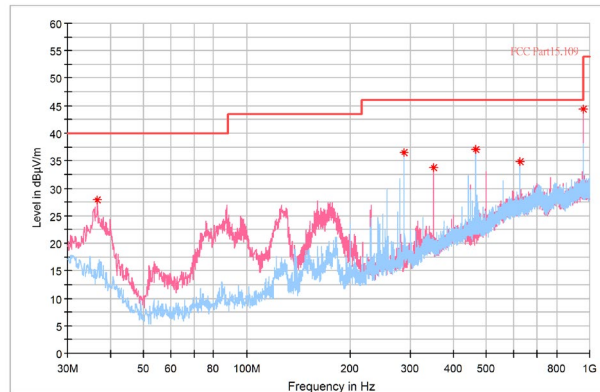
Figure 9. 30M-1GHz
