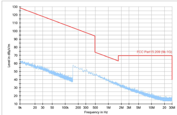
Figure 1. 9k-30MHz
