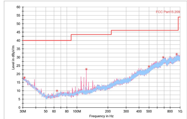
Figure 2. 30M-1GHz
