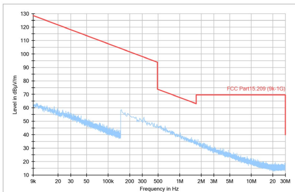
Figure 8. 9k-30MHz
