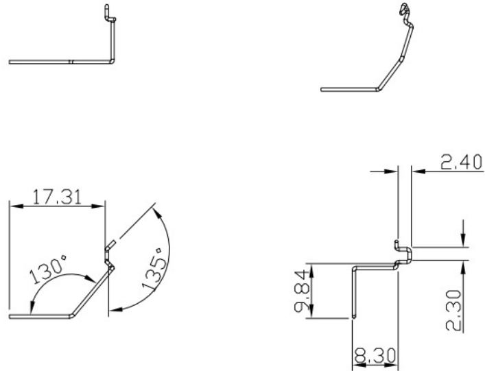
Figure 1 Physical dimension (mm)
