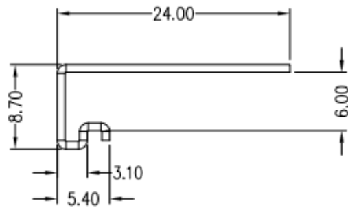
Figure 1 Physical dimension (mm)
