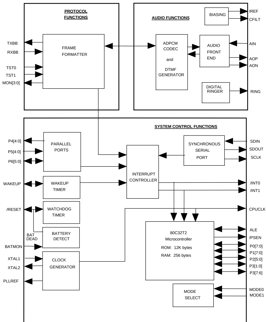
Figure 5. AMD ASIC - Internal Structure Diagram
