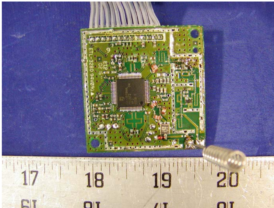
Antenna with Transmitter Metal Shield Removed View
