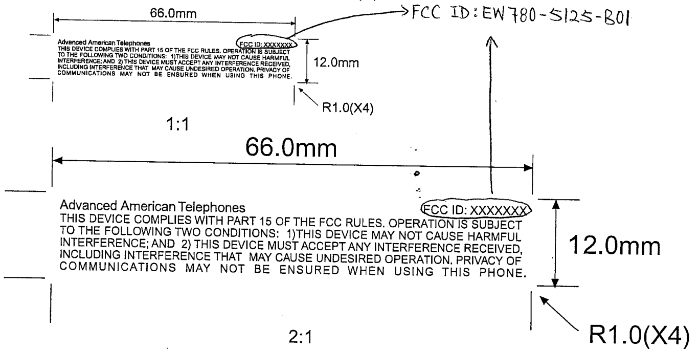
AT&T 1430 BASE BTMT- FCCID (PART15) Engrave (C)
