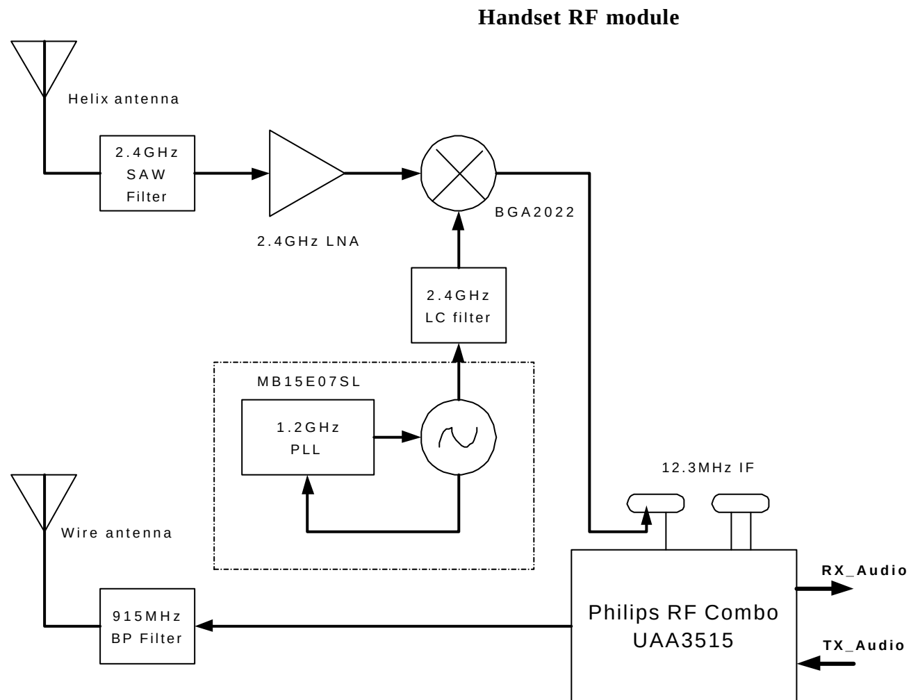
Figure 3. RF Circuits in Handset Unit
