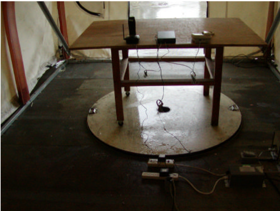
Base & Handset Conducted Emission - Rear View
