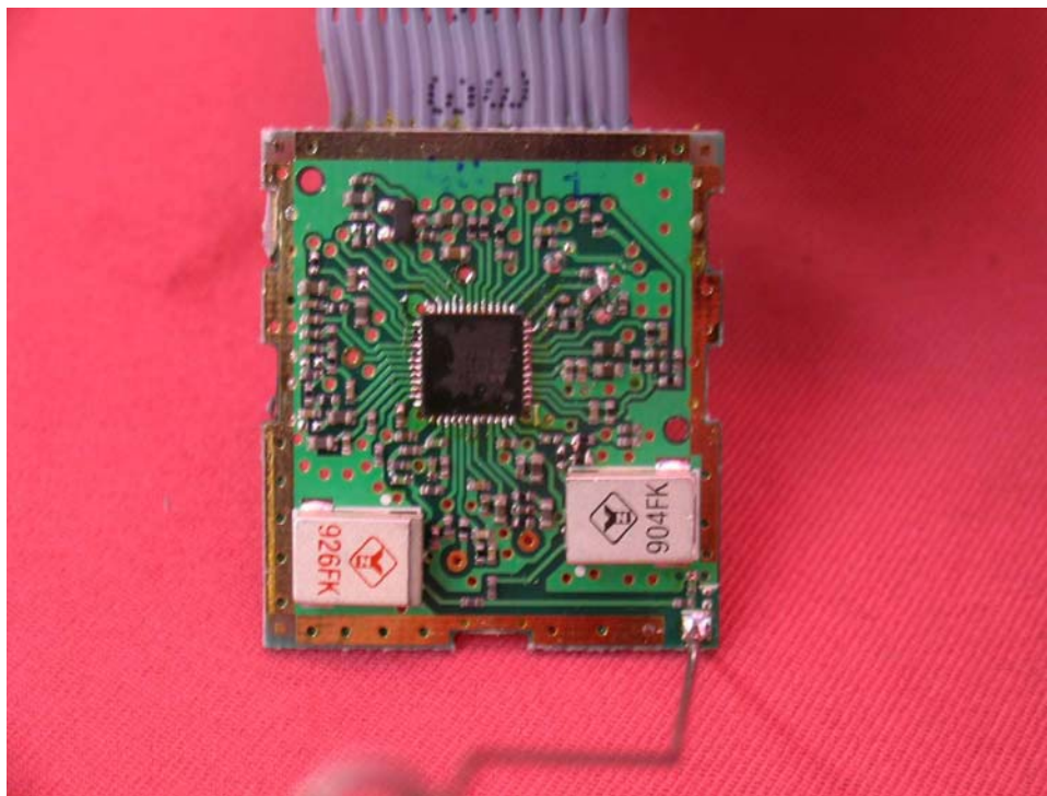
Base Oscillator PCB comp side
