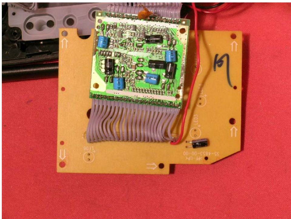
Base DAM PCB rear side (View 2)
