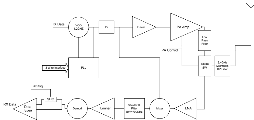
RF Block Diagram
