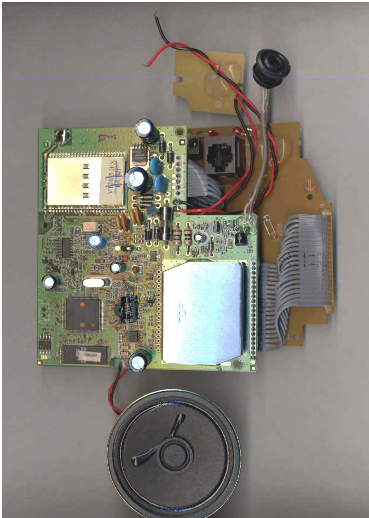
Vtech 2656 Base PCB
