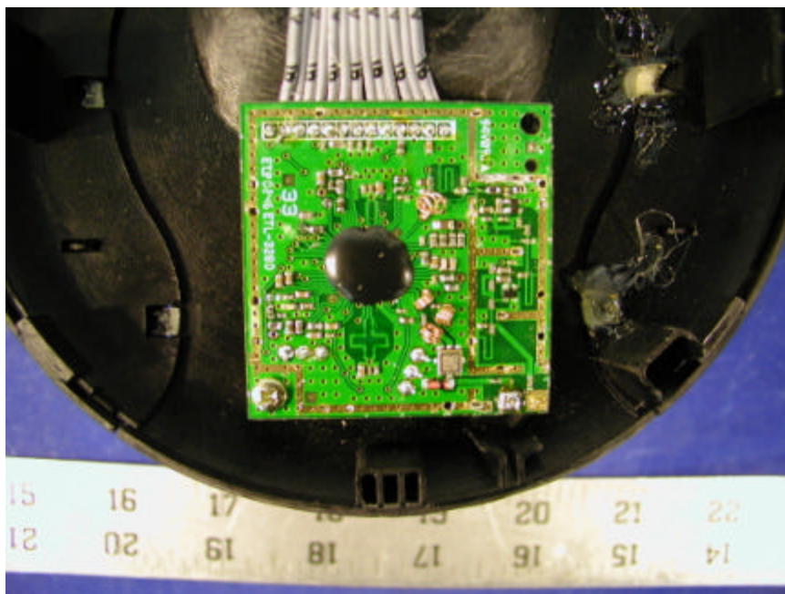
Base Transmitter with Housing
