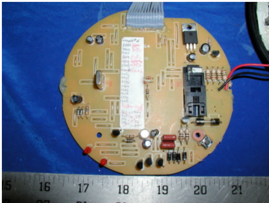
Base Main Board - Solder View
