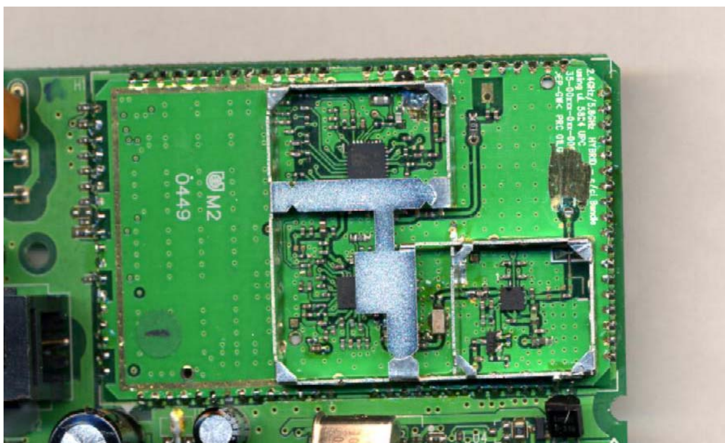
Vtech 5825 Base PCB (New Base RF)
