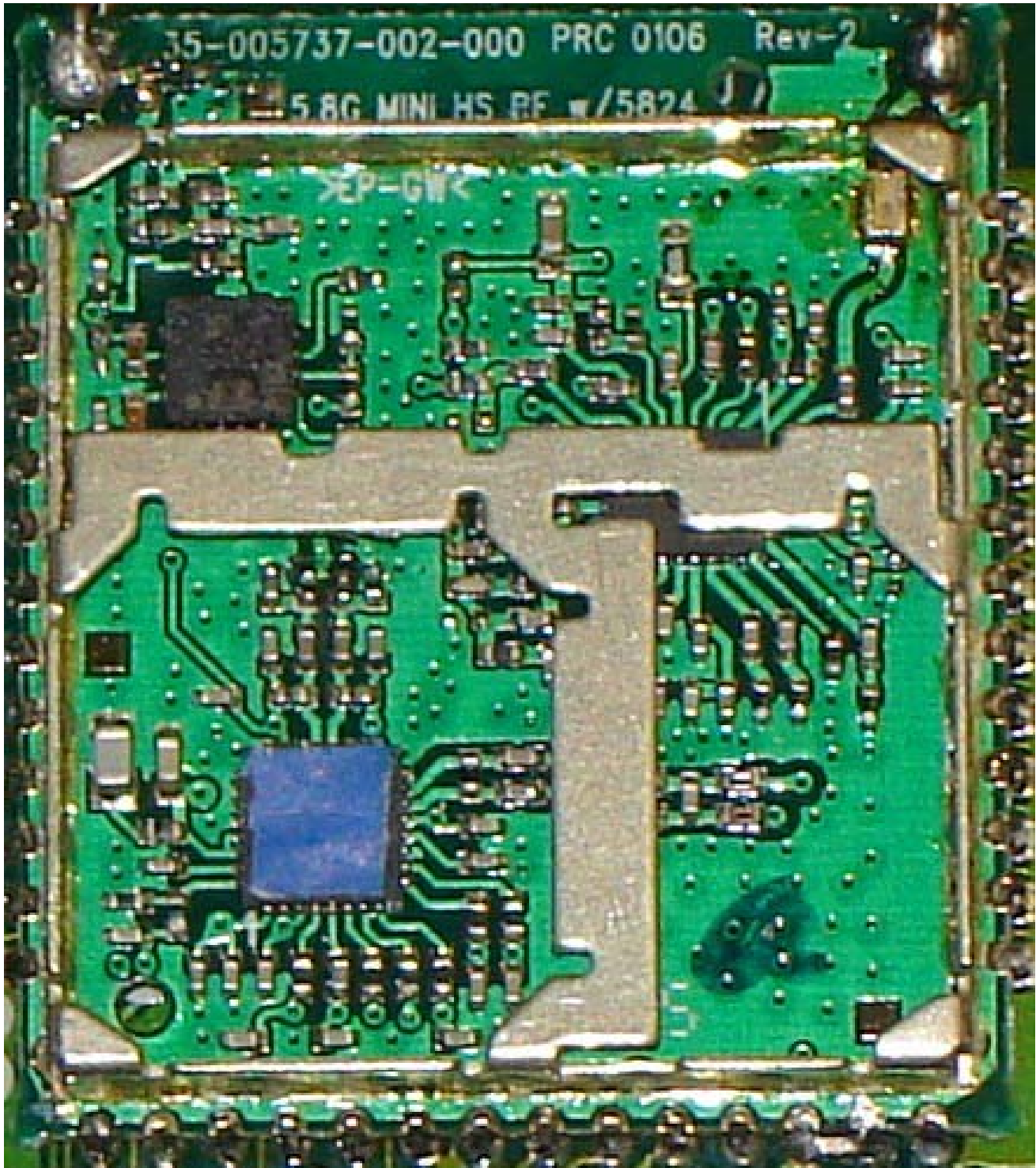
Vtech I6764 Handset RF – Internal Photo
