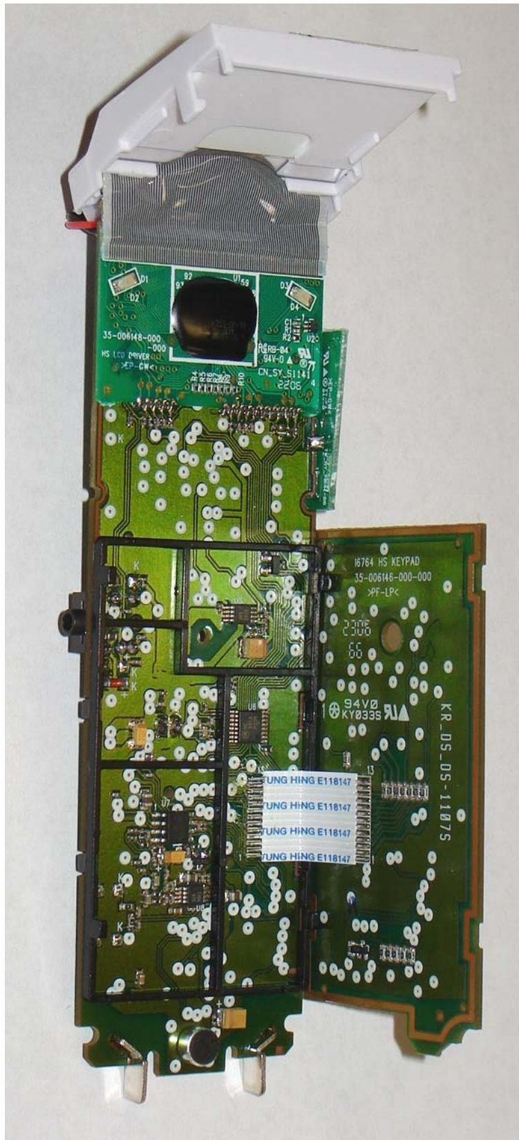
Vtech I6764 Handset PCB – Internal Photo
