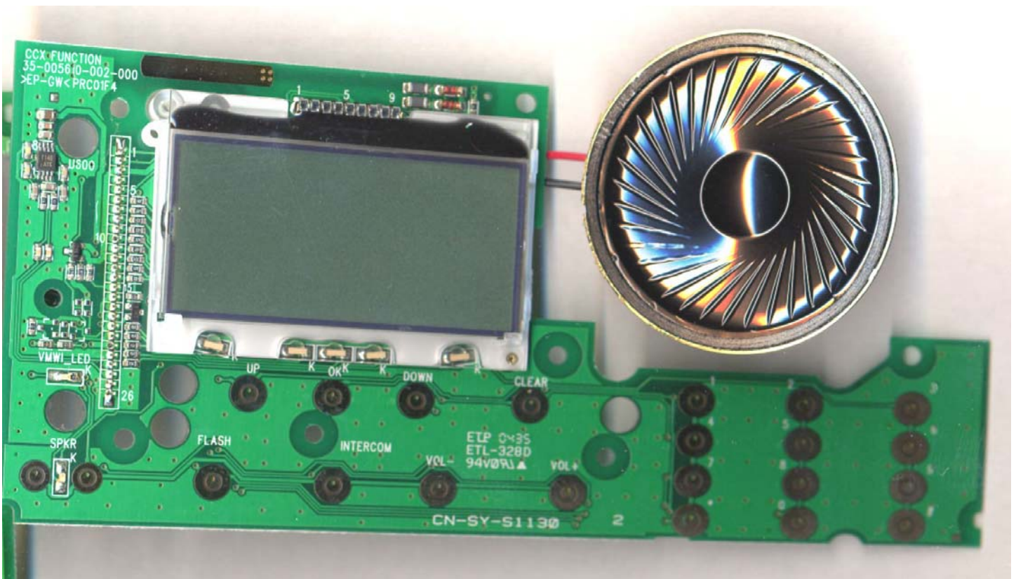
VTech 5871 Base PCB
