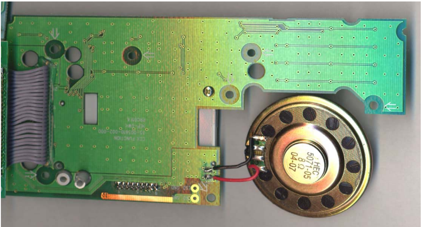
VTech 5871 Base PCB
