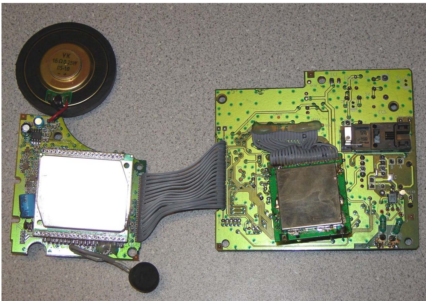
VTech mi6866 Base PCB (with Shield)
