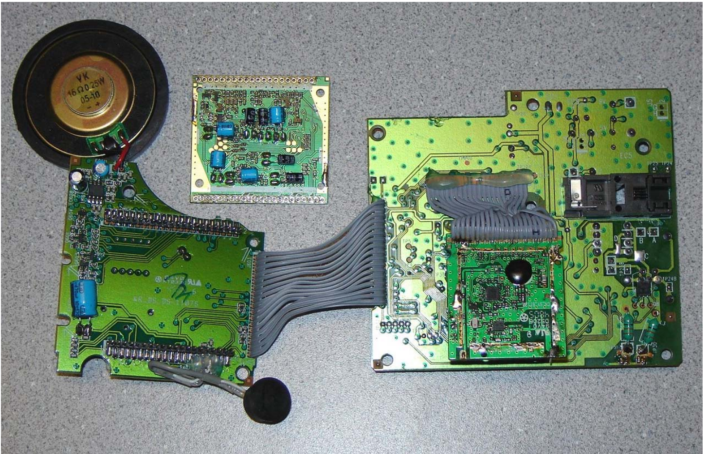
VTech mi6866 Base PCB (without Shield)
