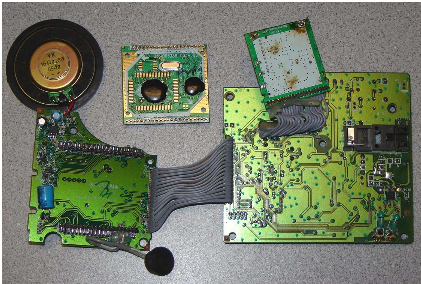
VTech mi6866 Base PCB (with Shield)
