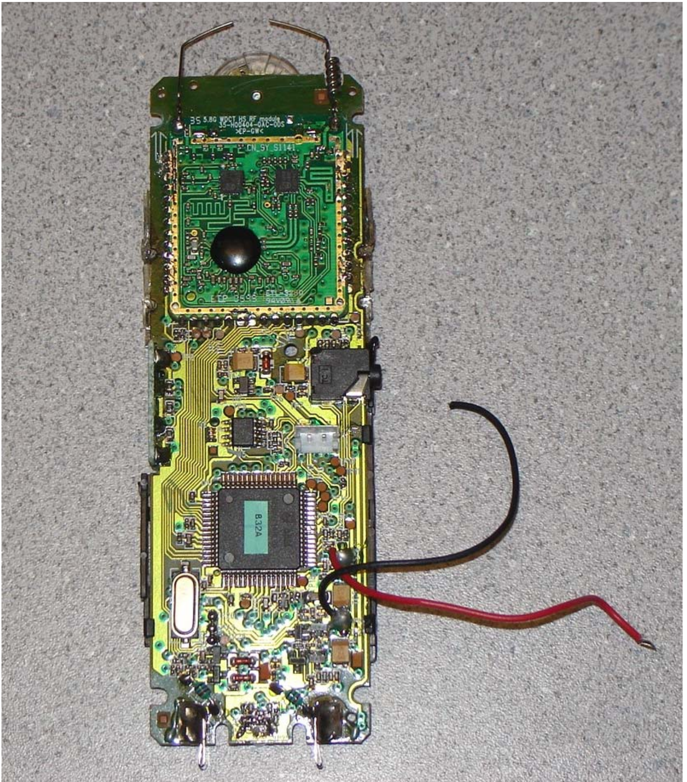
VTech mi6866 Handset PCB (without shield)
