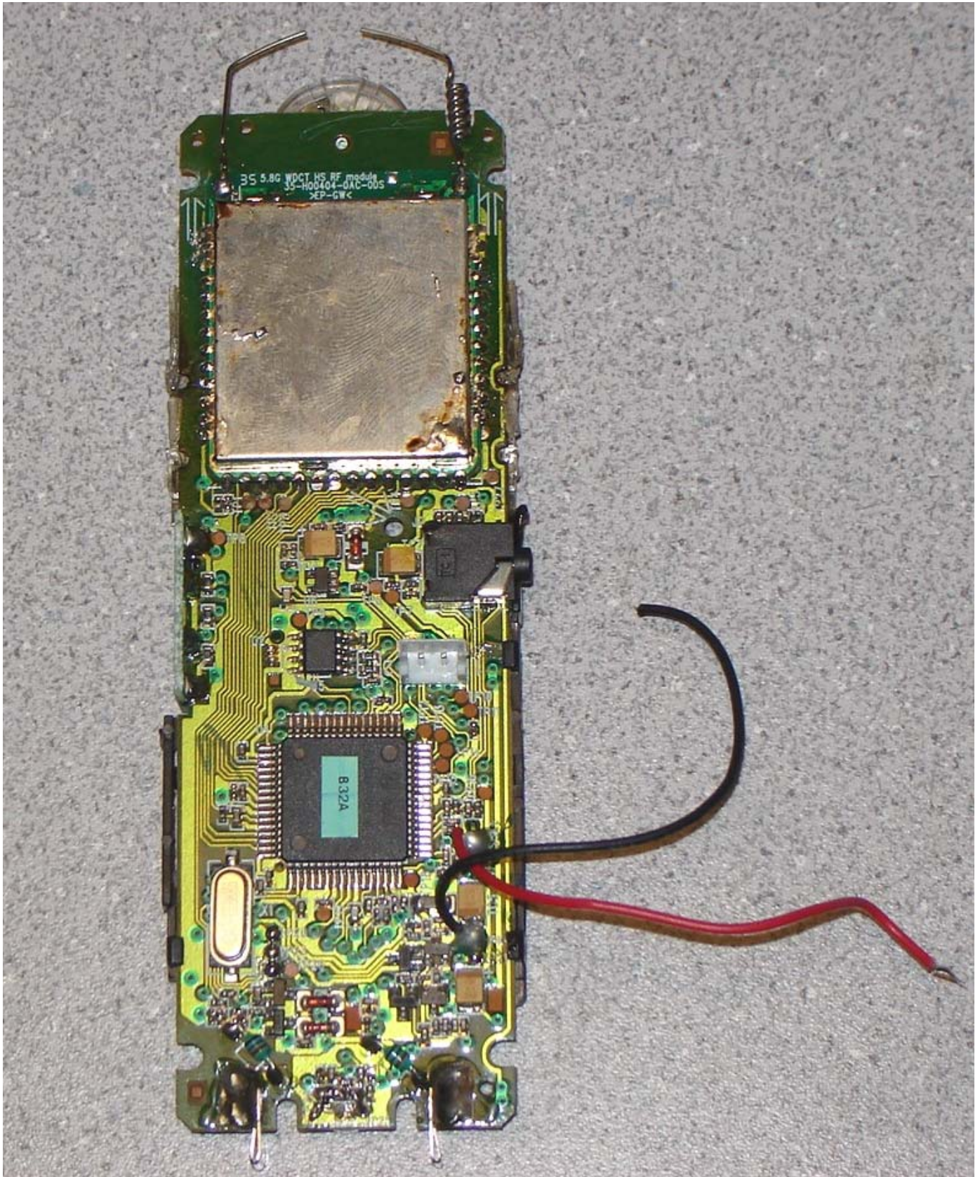
VTech mi6866 Handset PCB (with shield)
