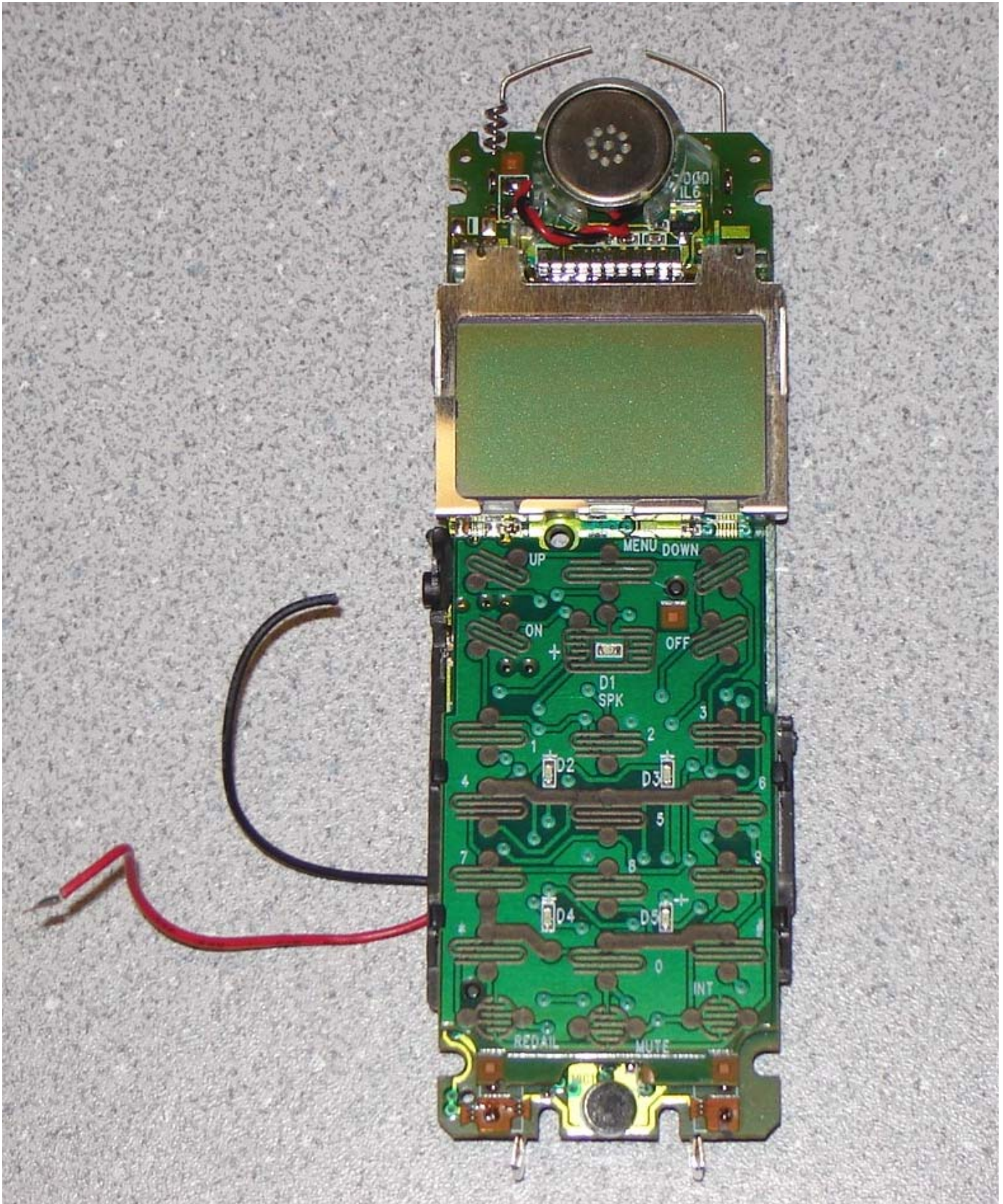
VTech mi6866 Handset PCB
