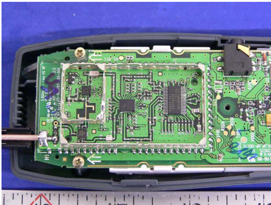
Handset – TX View
