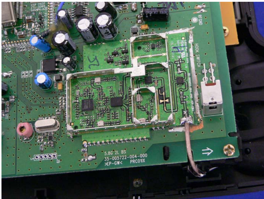
Base - Transmitter View
