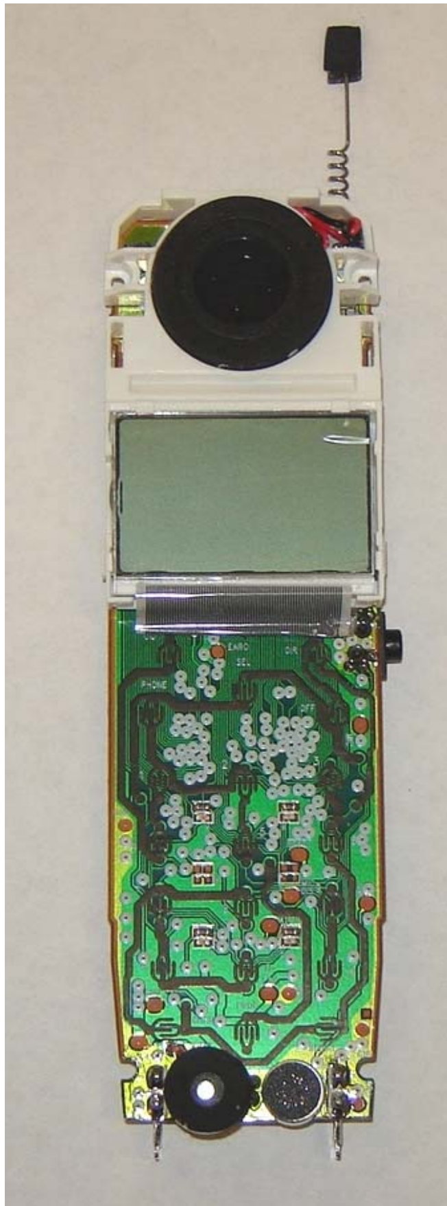
VTech ia5823 Handset PCB
