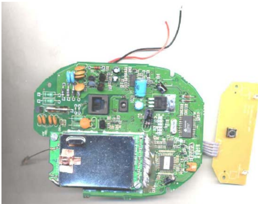
EUT – Component View I
