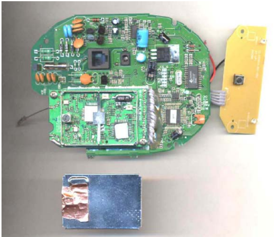
EUT – Component View II
