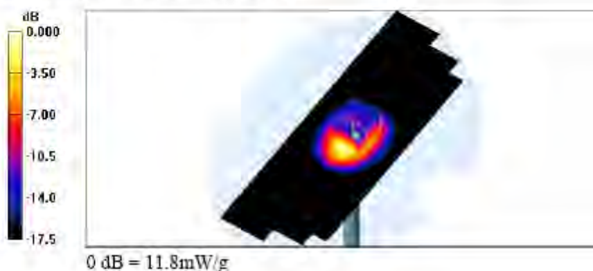
Head-Tissue-Simulating-Liquid 2GHz
