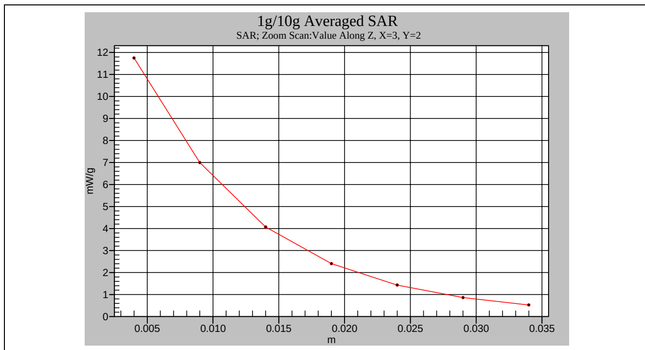
Head-Tissue-Simulating-Liquid 2GHz
