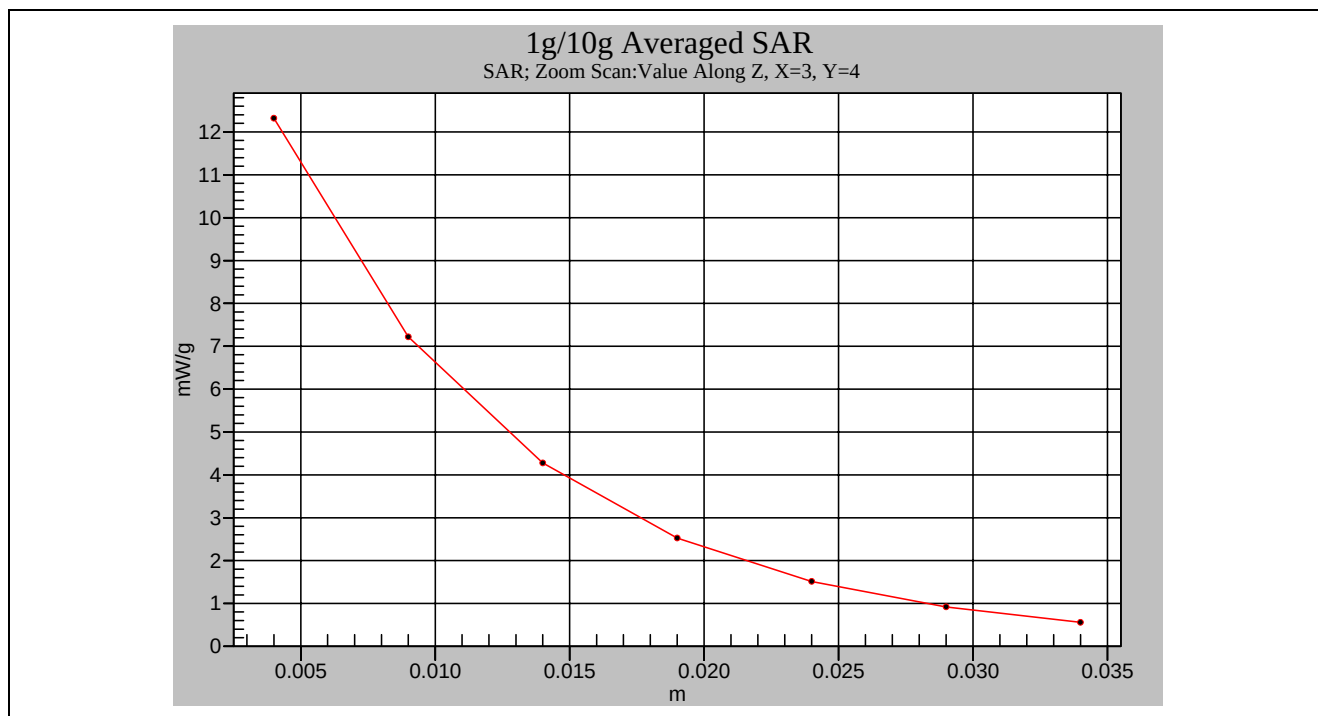
Body-Tissue-Simulating-Liquid 2GHz
