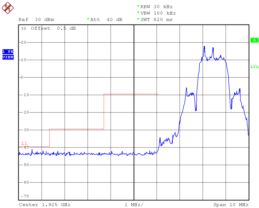
Plot 4B. Highest Channel Unwanted Emission Inside the Sub-Band (Traffic Carrier)
