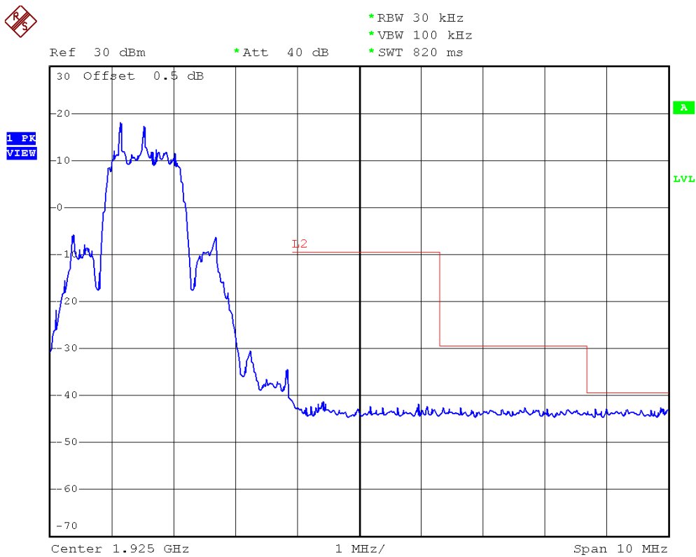
Plot 4A. Lowest Channel Unwanted Emission Inside the Sub-Band (Traffic Carrier)
