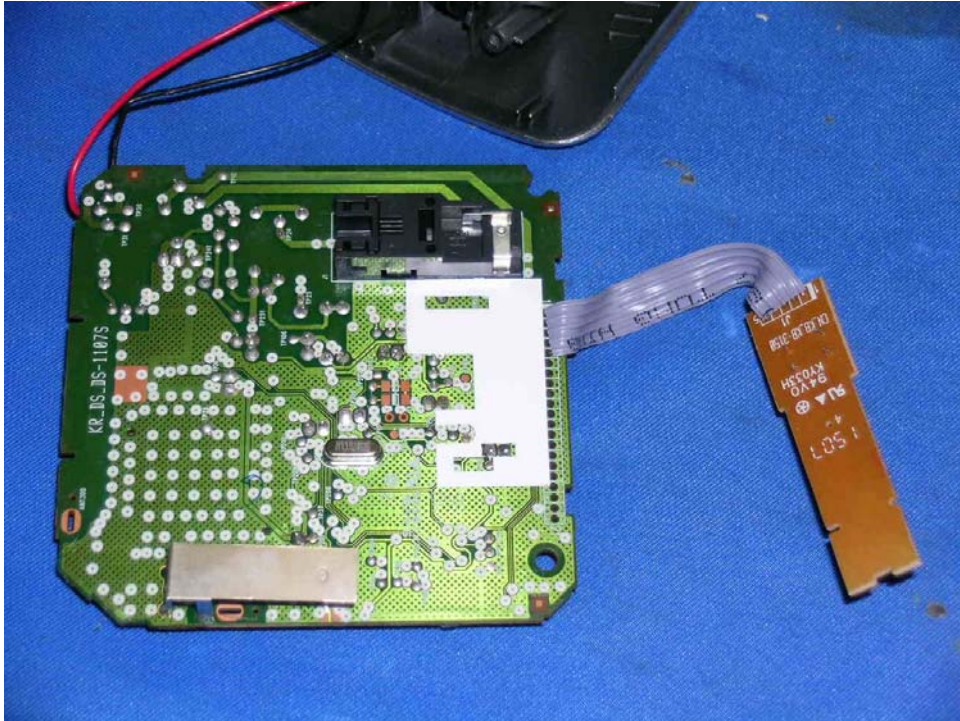
Base Unit Main PCB and Keypad solder side
