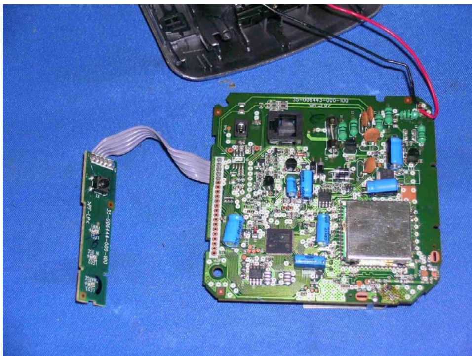
Base Unit Main PCB and Keypad comp side
