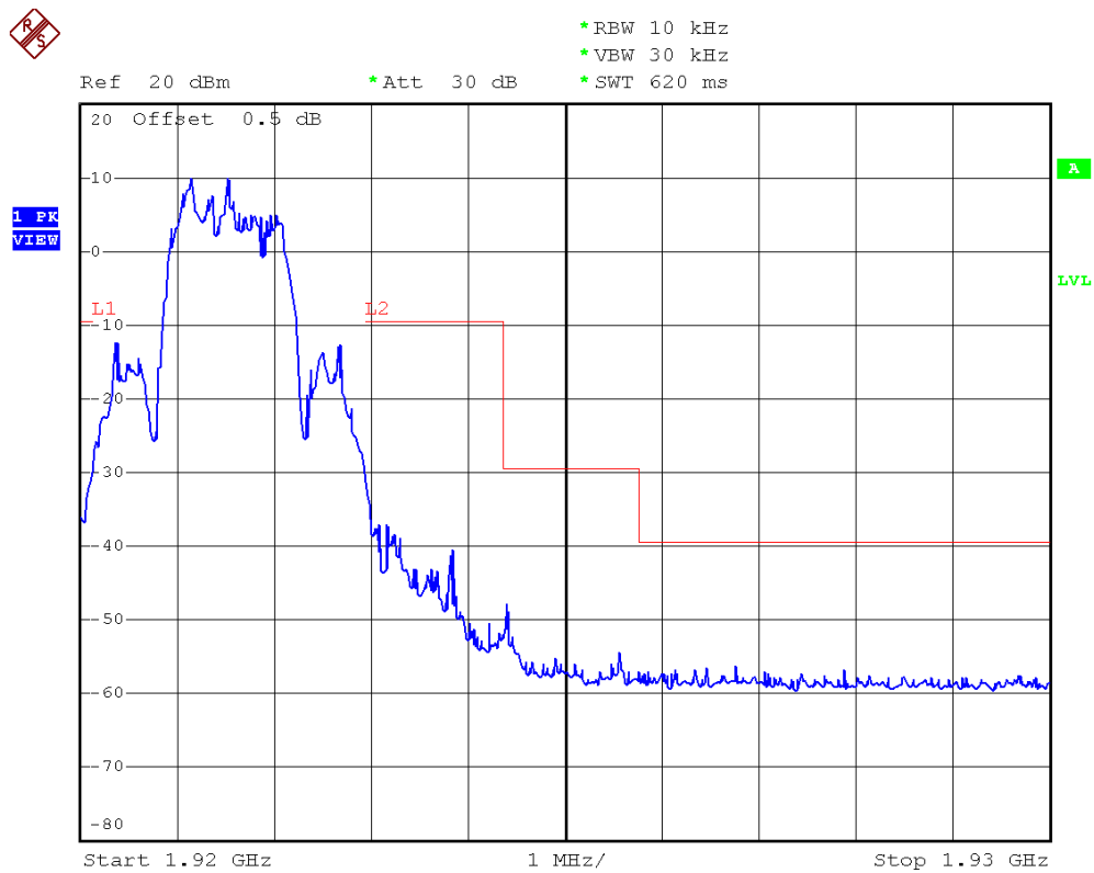
Plot 4A. Lowest Channel Unwanted Emission Inside the Sub-Band (Traffic Carrier)
