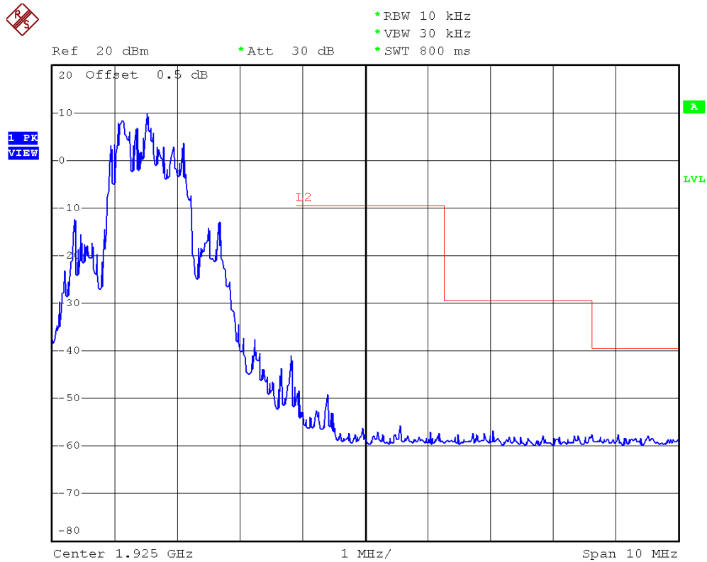
Plot 4C. Lowest Channel Unwanted Emission Inside the Sub-Band (Dummy Carrier)
