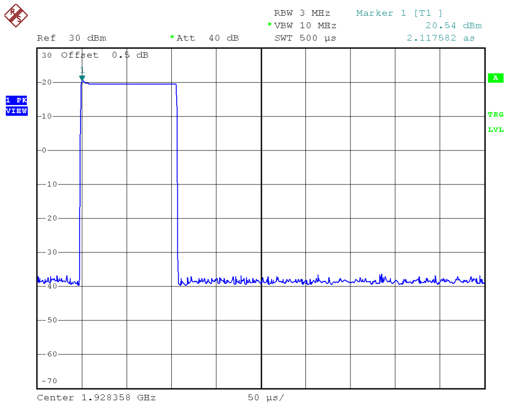
Plot 2D. Highest Channel Peak Transmit Power (Dummy Carrier)
