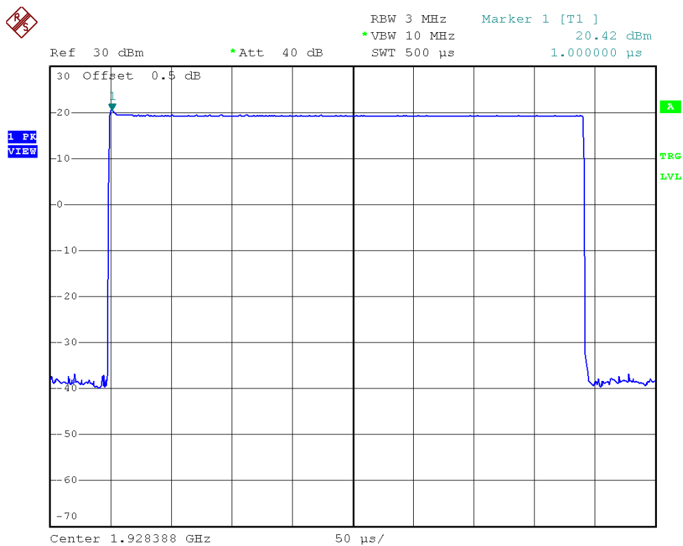
Plot 2B. Highest Channel Peak Transmit Power (Traffic Carrier)
