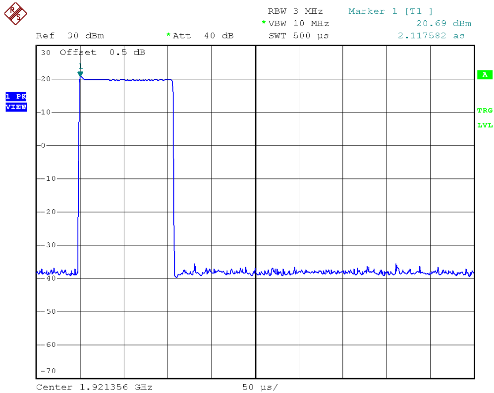
Plot 2C. Lowest Channel Peak Transmit Power (Dummy Carrier)
