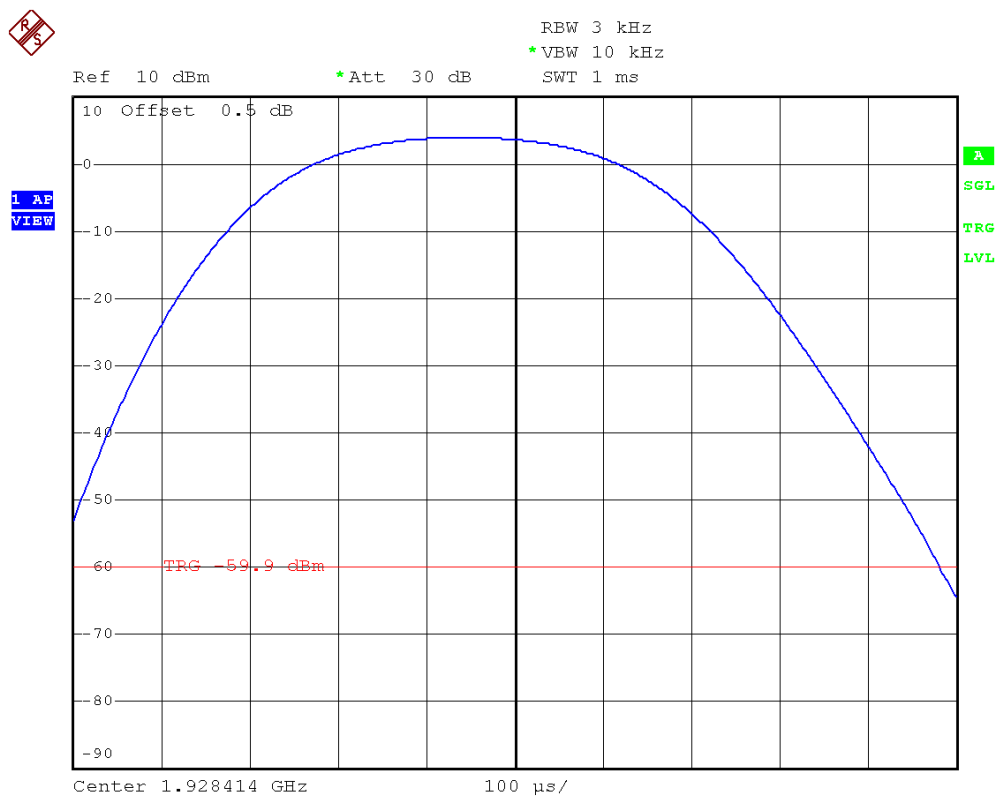
Plot 3B. Highest Channel Power Spectral Density (Traffic Carrier)
