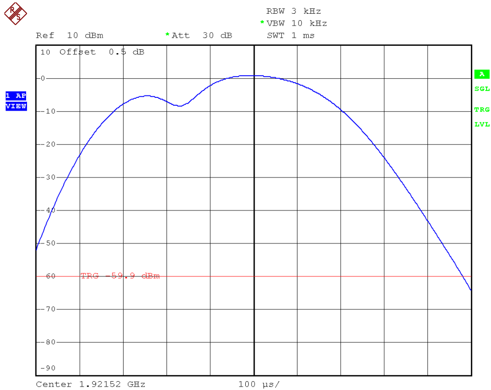
Plot 3A. Lowest Channel Power Spectral Density (Traffic Carrier)
