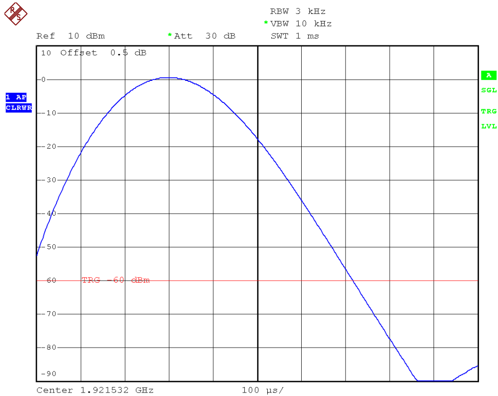
Plot 3C. Lowest Channel Power Spectral Density (Dummy Carrier)
