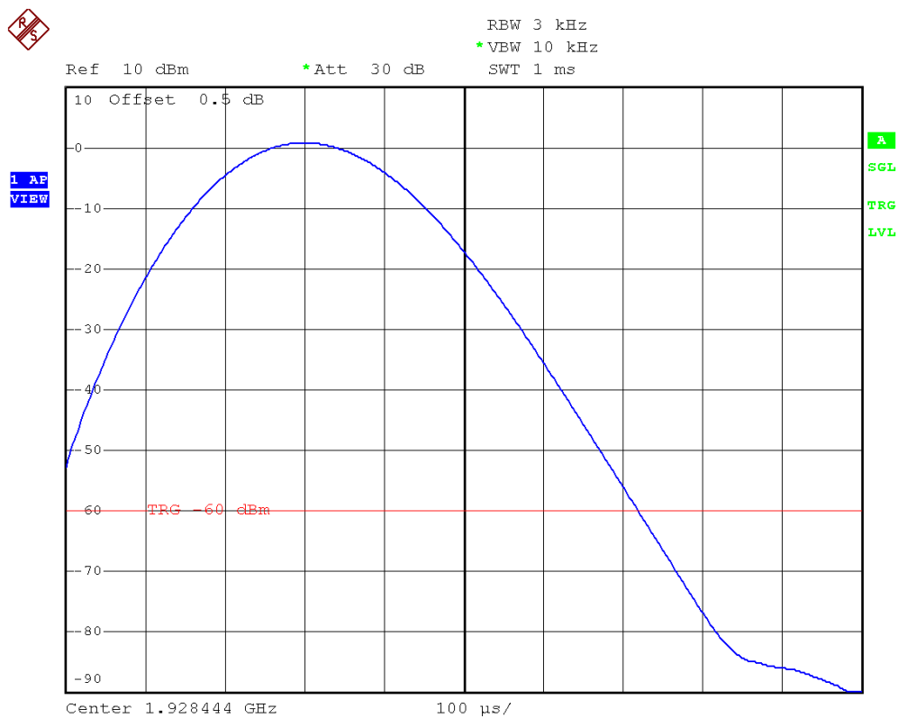
Plot 3D. Highest Channel Power Spectral Density (Dummy Carrier)
