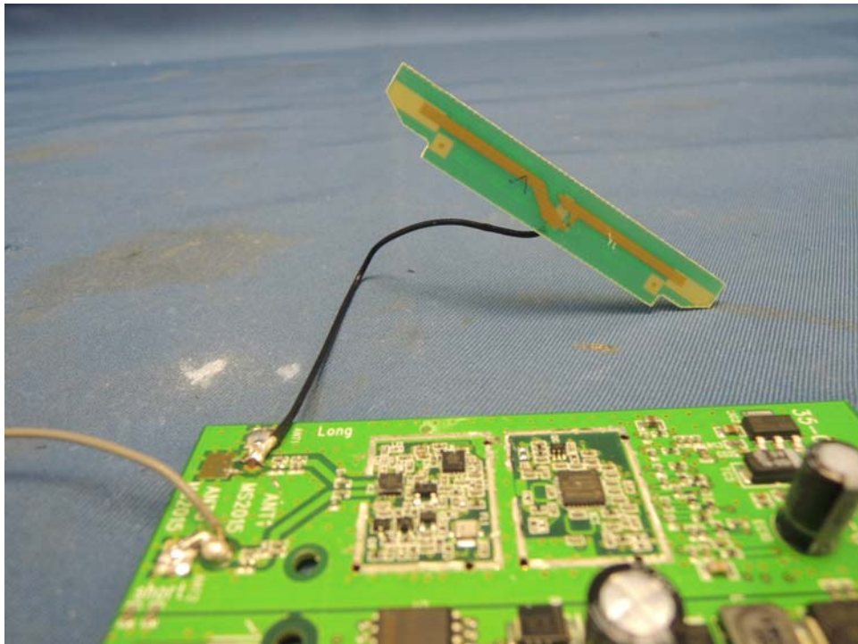
Deskset Antenna 2 (View 2)
