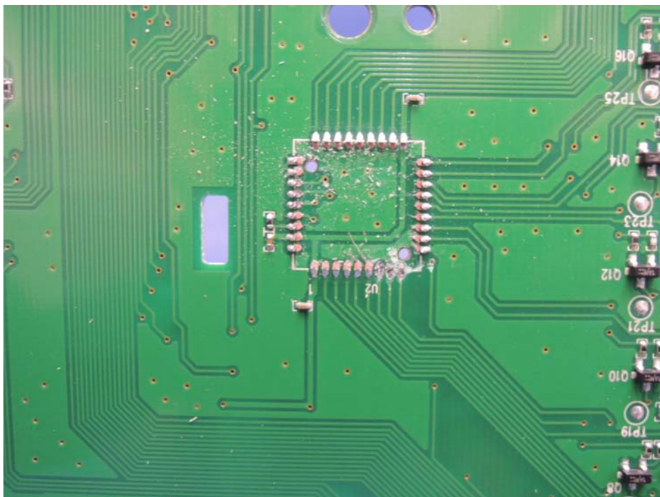
Deskset Keypad rear side (View 3)
