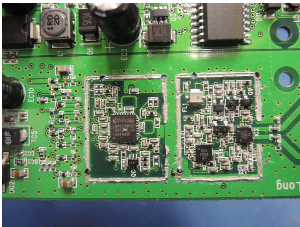
Deskset Oscillator PCB comp side
