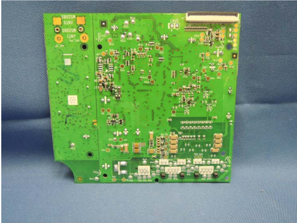
Deskset Main PCB solder side
