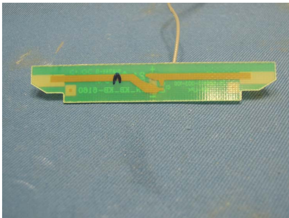
Deskset Antenna 1 (View 2)
