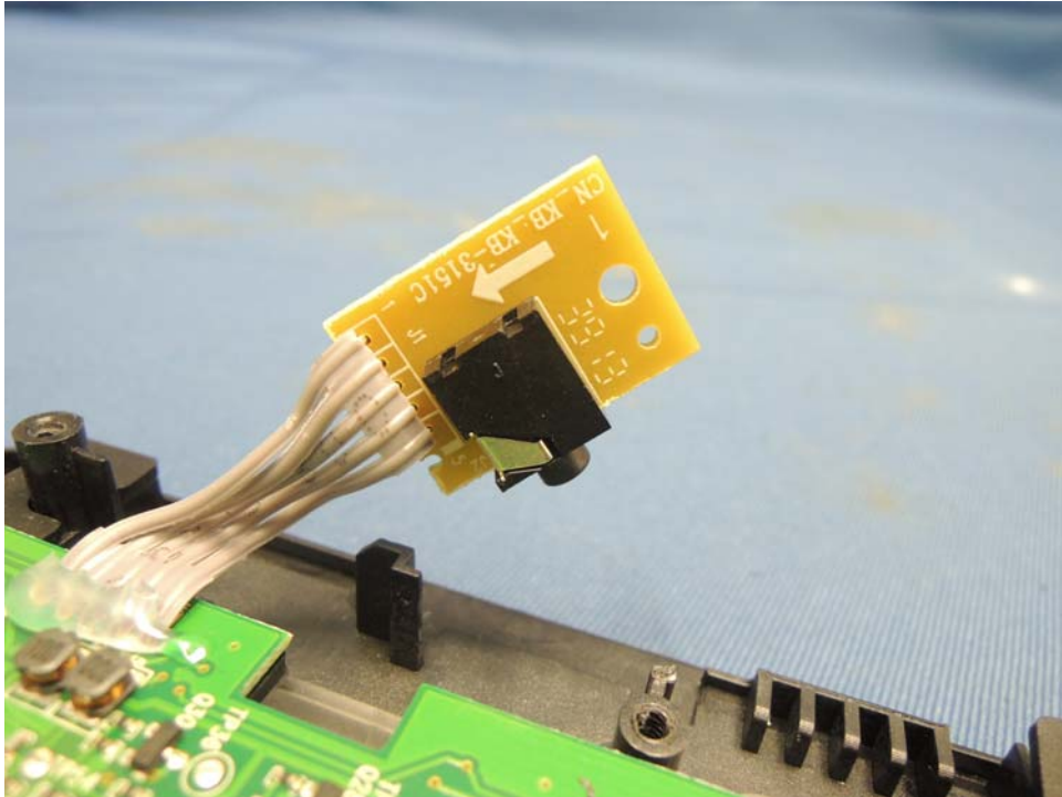
Deskset AC Jack front side
