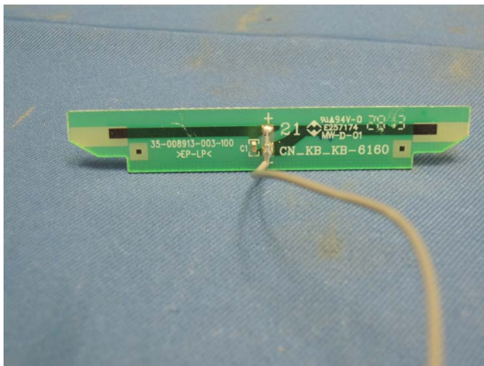
Deskset Antenna 1 (View 1)
