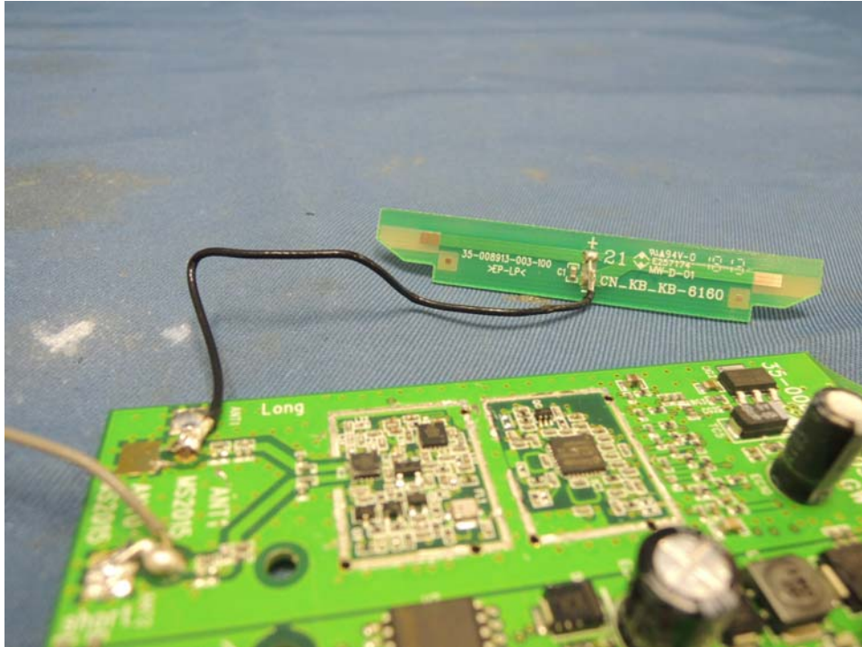
Deskset Antenna 2 (View 1)
