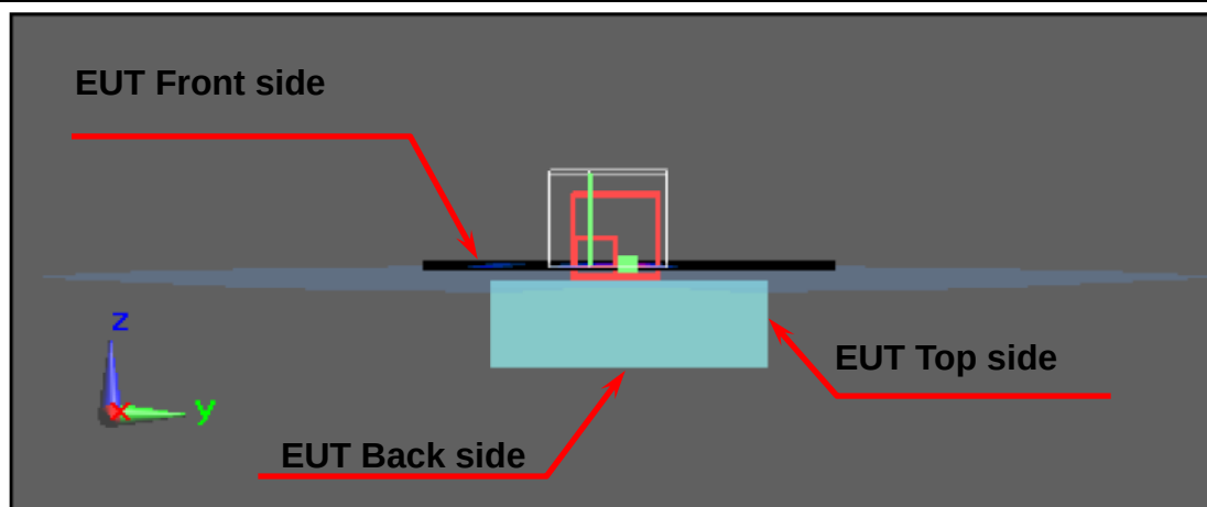
Figure 3. Muscle SAR Test Setup (Flat Section)
