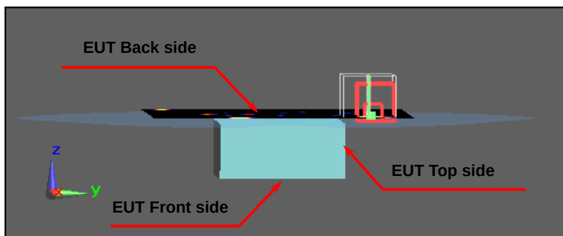
Figure 5. Muscle SAR Test Setup (Flat Section)
