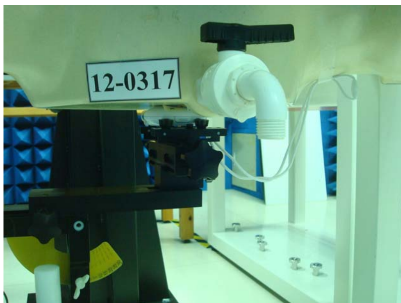
Figure 2. Brain SAR Test Setup (Flat Section)
