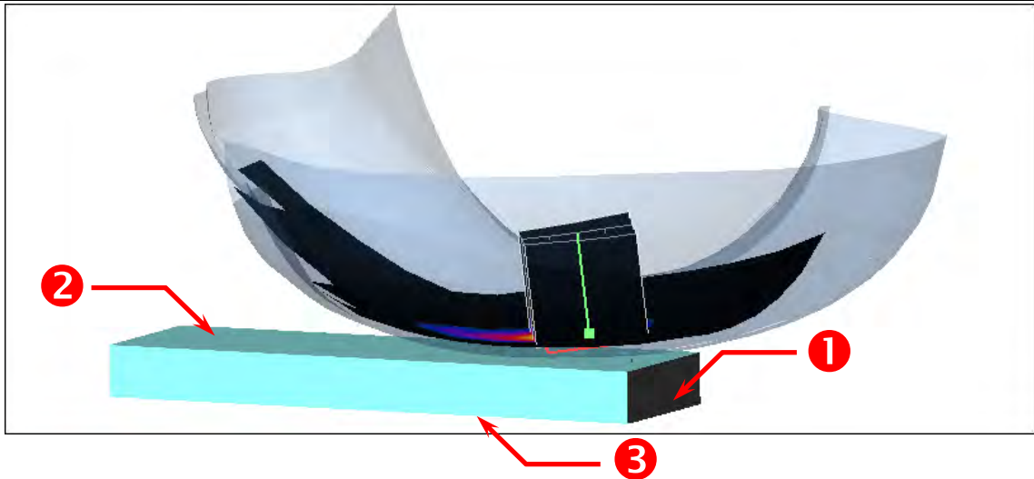
Figure 4. Left Head SAR Test Setup (Cheek)
