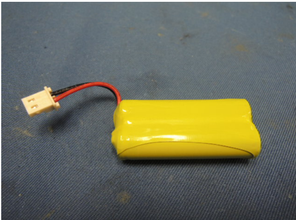
Figure 10 – 2.4V 750mAh Ni-MH Coslight rechargeable battery back view
