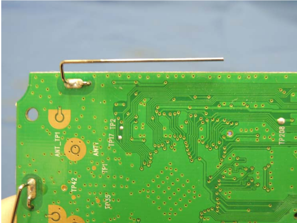
Base Unit – DECT Antenna 2
