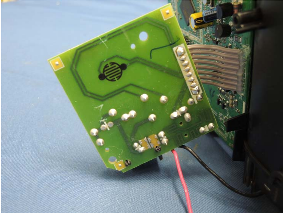
Base Unit Telephone Line and AC Jack rear side
