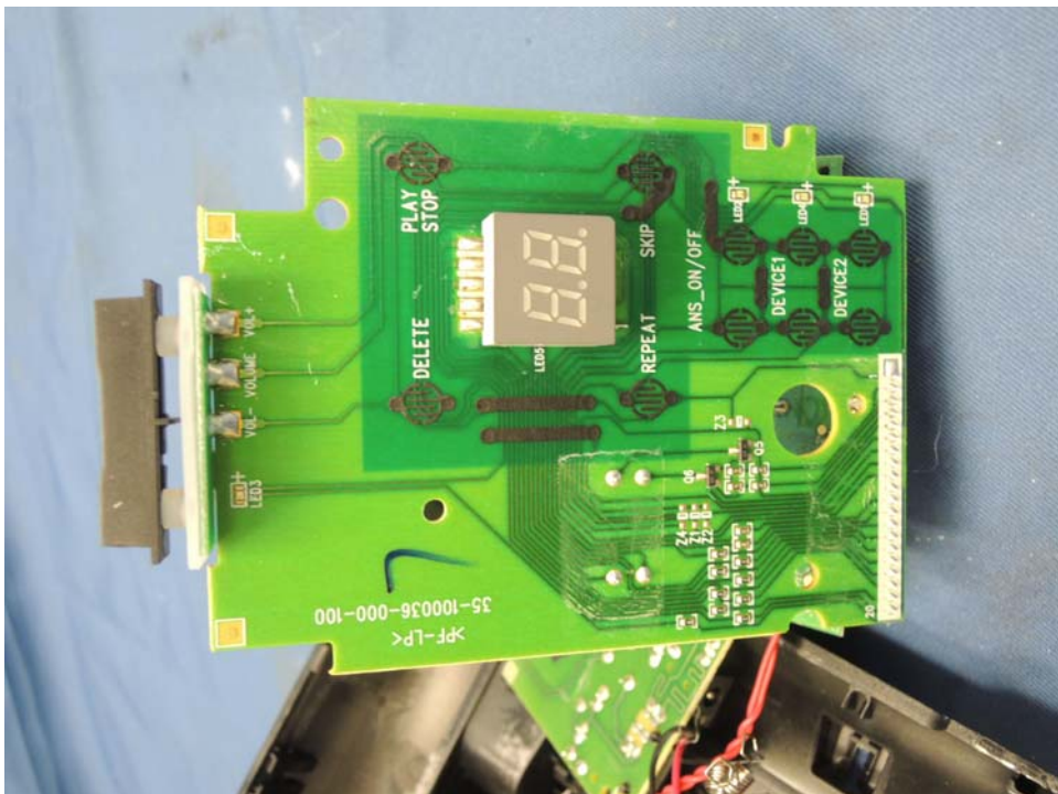
Base Unit DAM front side (View 1)
