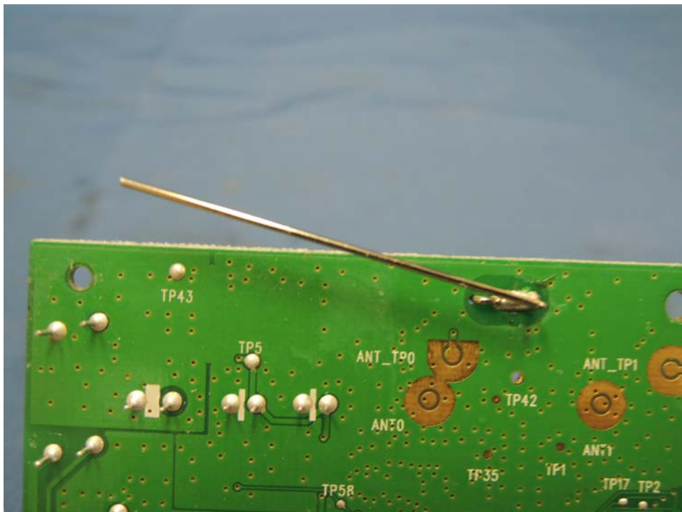
Base Unit – DECT Antenna 1
