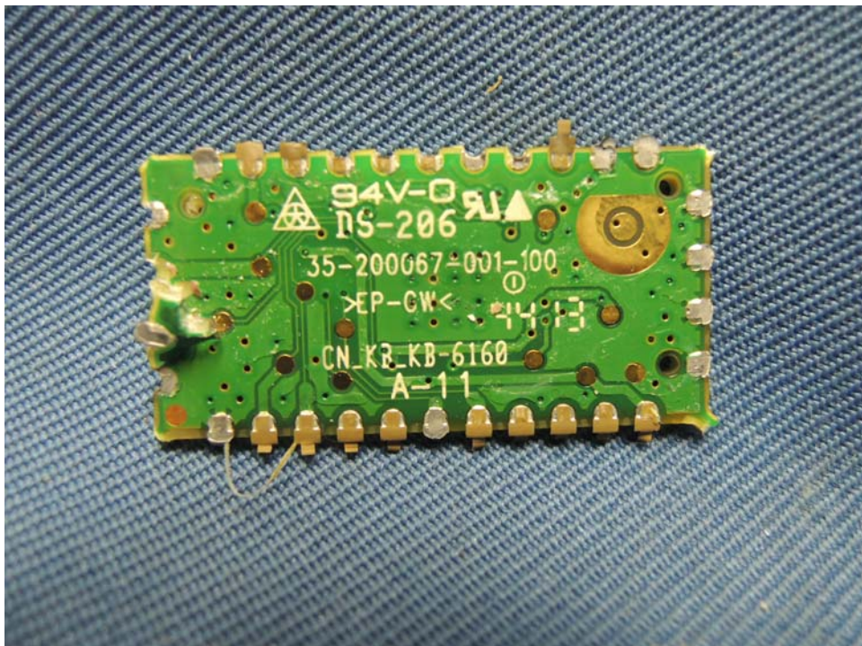
Base Unit Bluetooth RF Module solder side
