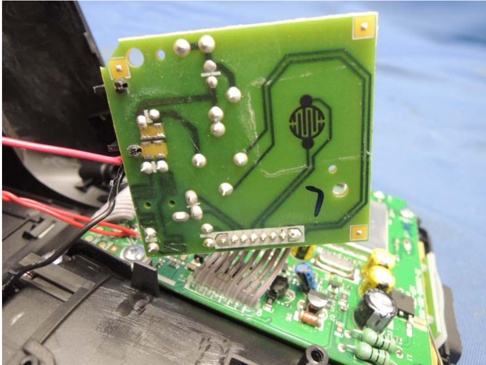
Base Unit Telephone Line and AC Jack rear side (View 2)
