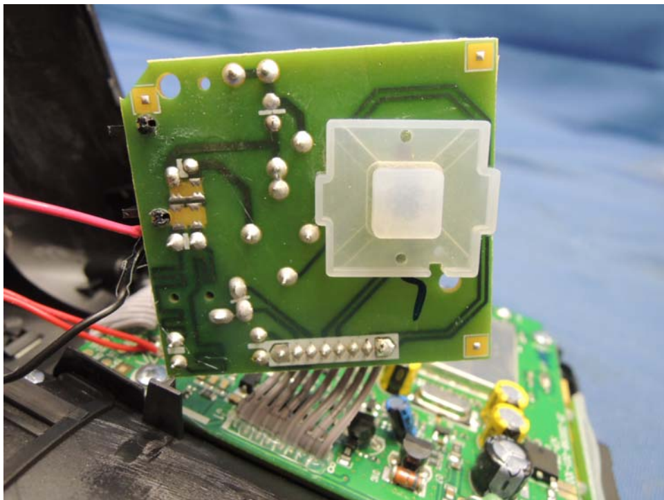
Base Unit Telephone Line and AC Jack rear side (View 1)
