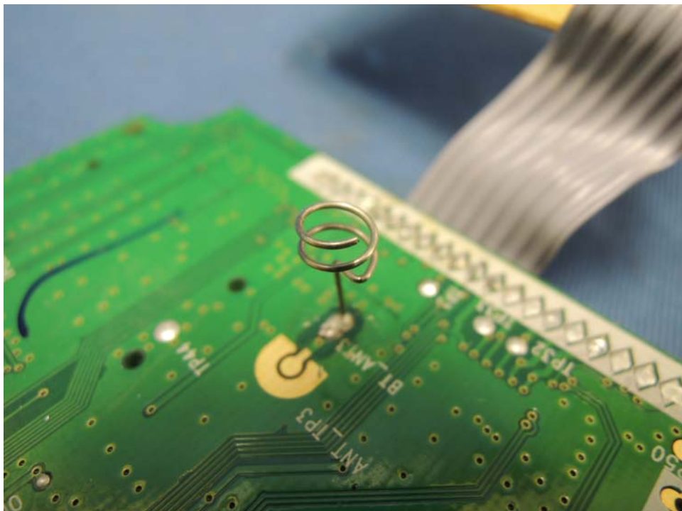
Base Unit – Bluetooth Antenna
