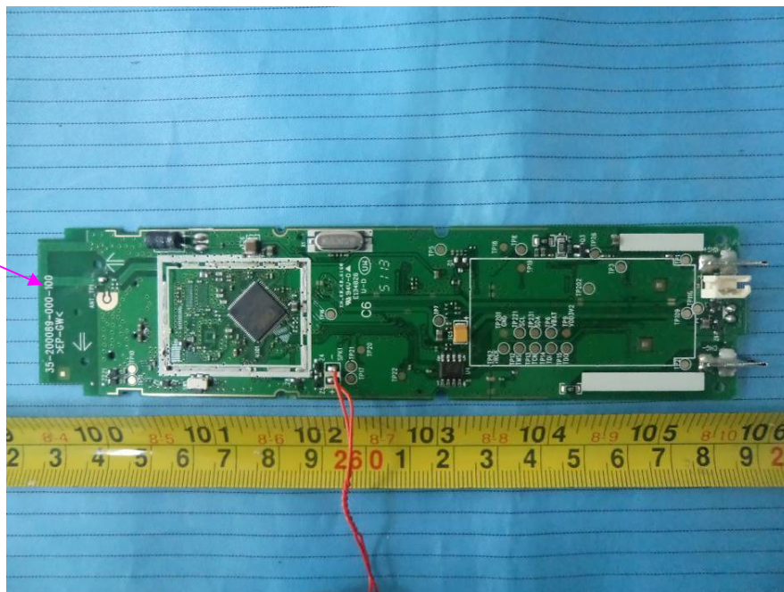
EUT – Main Board Top Shielding off View (1# Handset)
