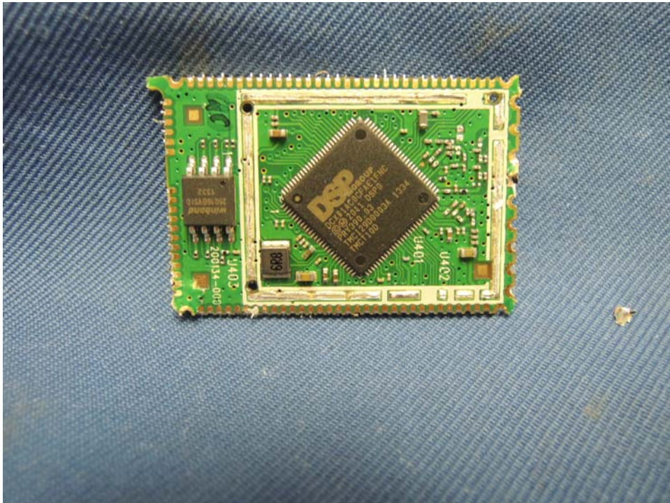
Handset RF PCB component side (View 1)
