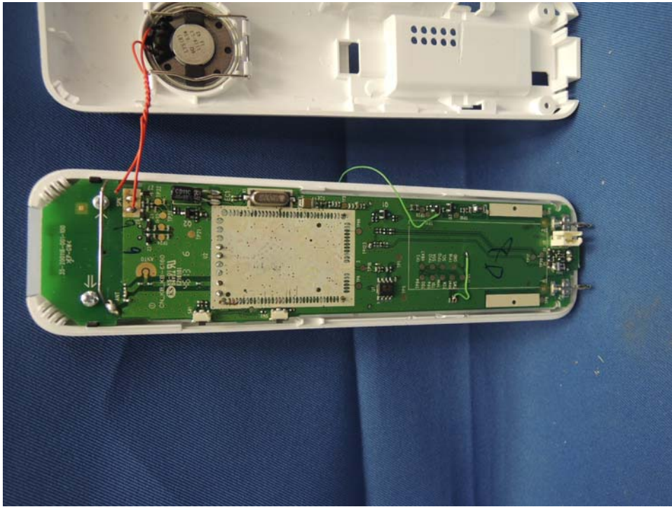
Handset Main PCB component side (View 4)
