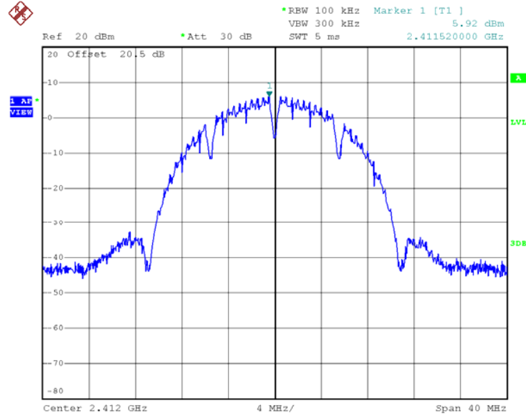
802.11b, Lowest channel
