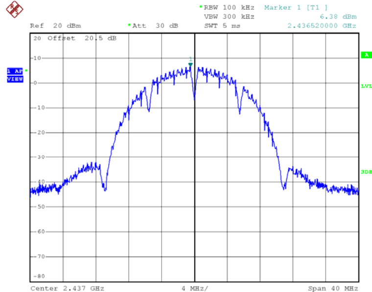
802.11b, Middle channel
