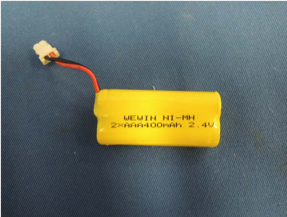
Figure 3 – 2.4V 400mAh Ni-MH Wewin rechargeable battery front view
