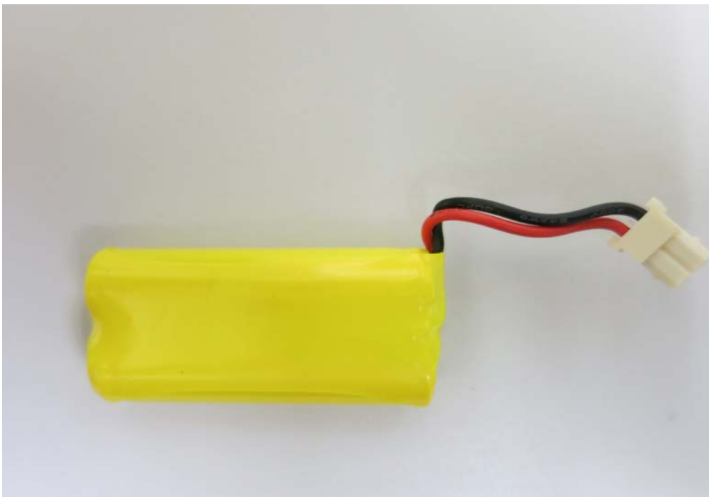
Figure 8 – 2.4V 400mAh Ni-MH Wewin rechargeable battery back view
