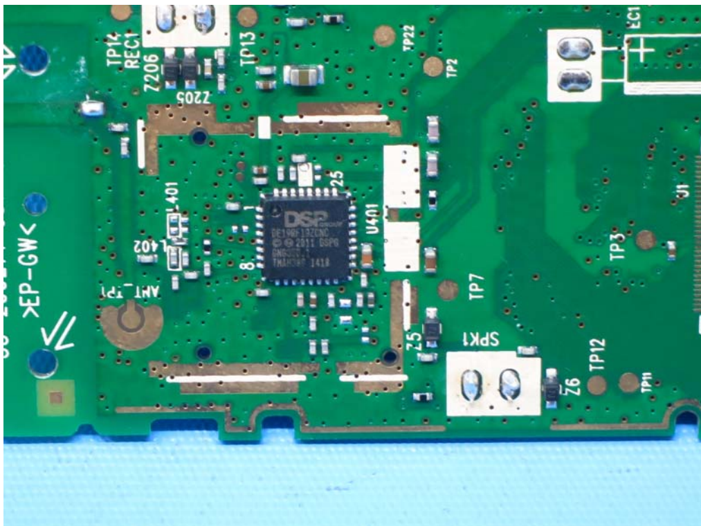
Handset Oscillator PCB comp side
