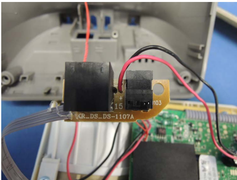
Base Unit DC Jack PCB comp side
