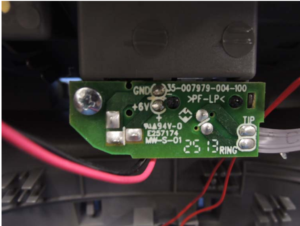
Base Unit DC Jack PCB solder side
