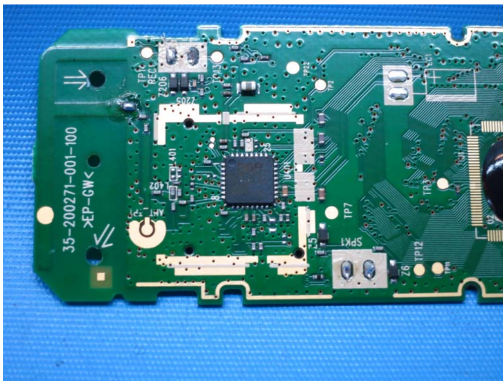
Handset Antenna
