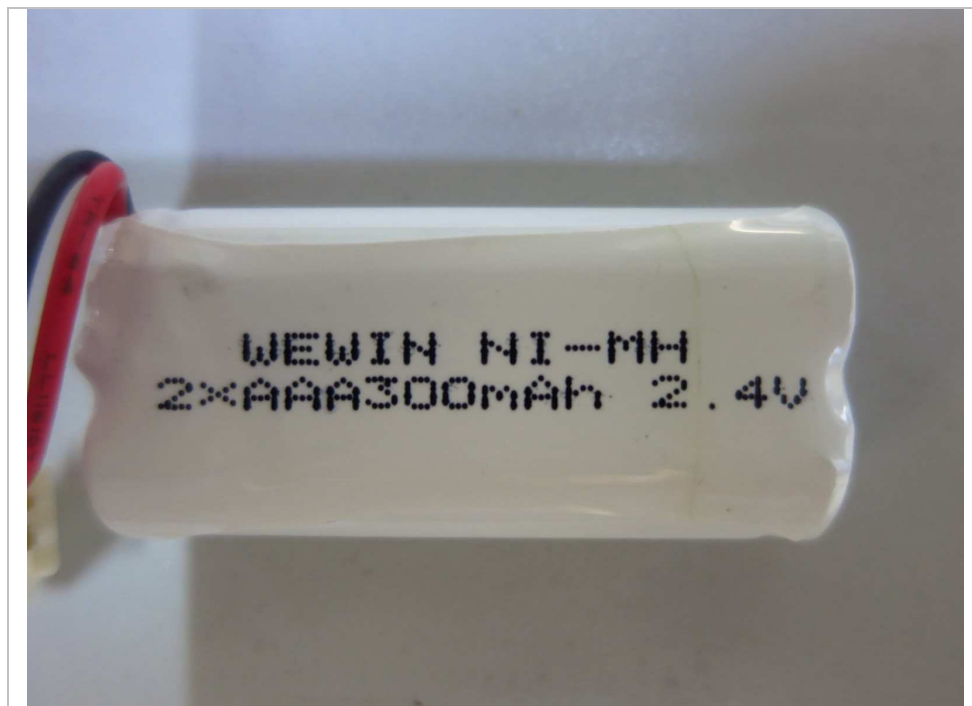
Figure 7 – 2.4V 300mAh Ni-MH Wewin rechargeable battery front view
