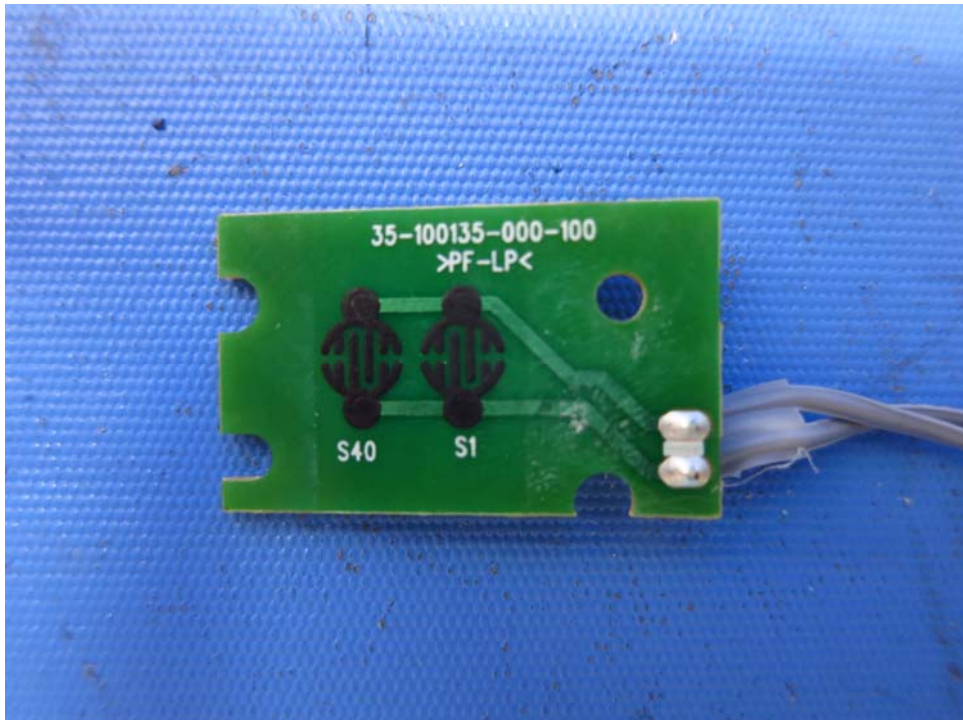
Base Unit – Handset Locator PCB solder side
