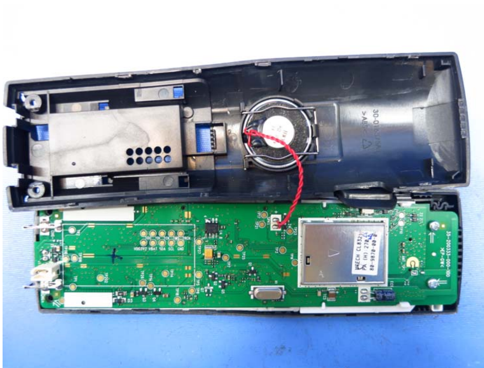
Handset assembly
