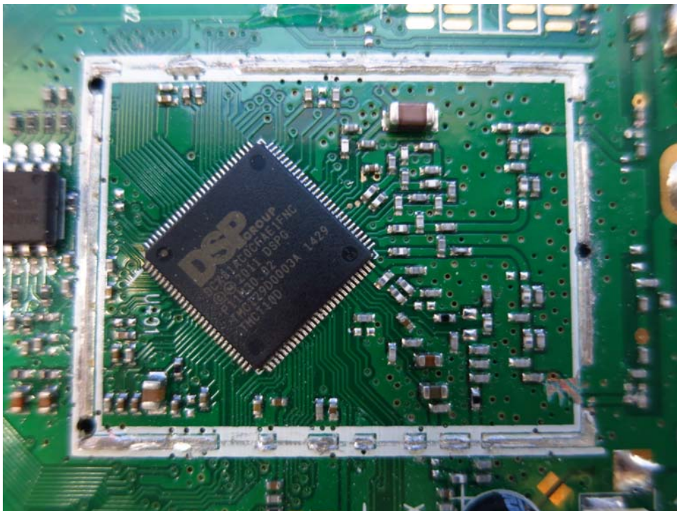
Base Unit – DECT Oscillator PCB comp side
