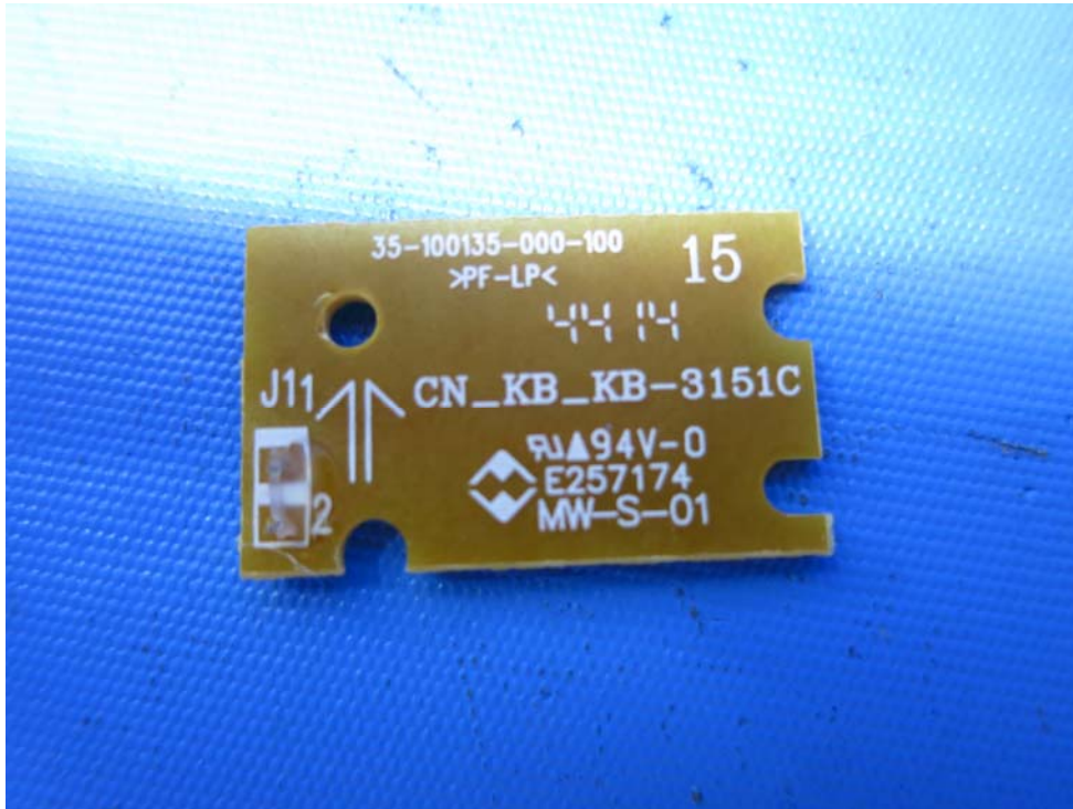
Base Unit – Handset Locator PCB comp side
