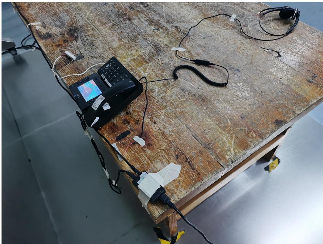
Conducted Emissions Side View For POE
