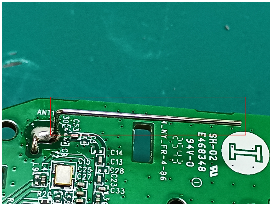
Zigbee ANT
