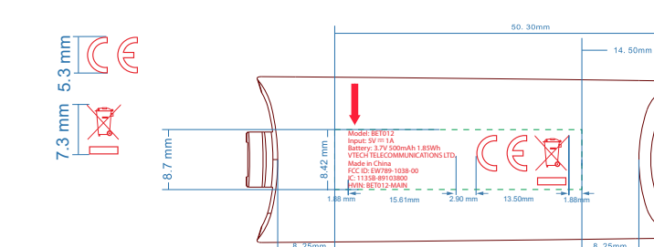
L side inner silkscreen
