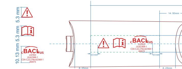
R side inner silkscreen
