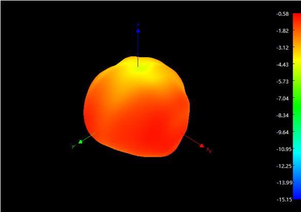
3D Radiation Pattern @ 2440 MHz
